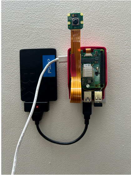
FIGURE 5. Deployed hardware — the exact rig on which every measurement in Section VI was taken. Components visible in the photograph: Raspberry Pi 5 (16 GB, in a red active-cooled case), Hailo-8L AI HAT+ (13 TOPS), Raspberry Pi Camera Module v3 with its CSI-2 ribbon cable, and a 1 TB Crucial SATA SSD in a USB 3 enclosure. Total assembled BOM US$450–500; board power under deployed concurrent inference load is 5.89 \pm 1.43 W (Section VI-J).
