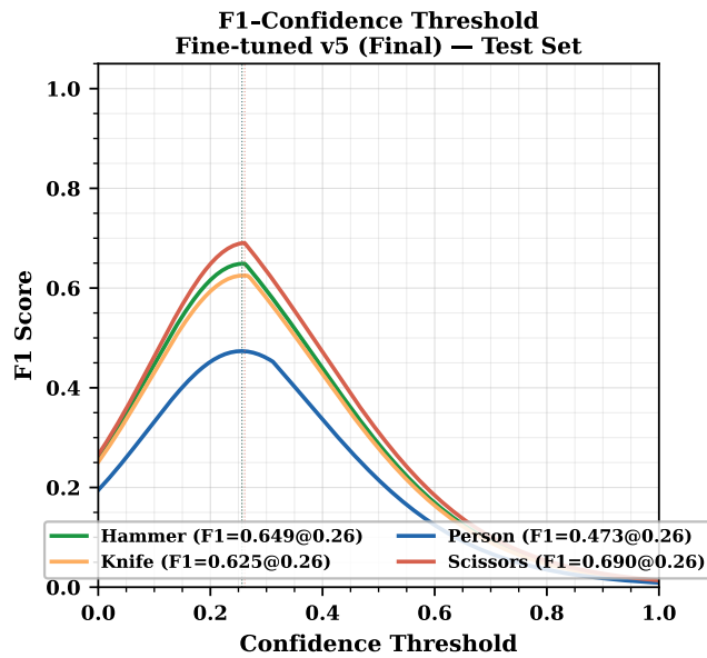
FIGURE 18. Per-class F1 score versus confidence threshold. All four classes peak in the 0.25–0.27 band, matching YOLO’s default threshold and eliminating the need for manual per-class tuning at deployment. Scissors reaches the highest peak F1 (0.690); Person the lowest (0.473).
